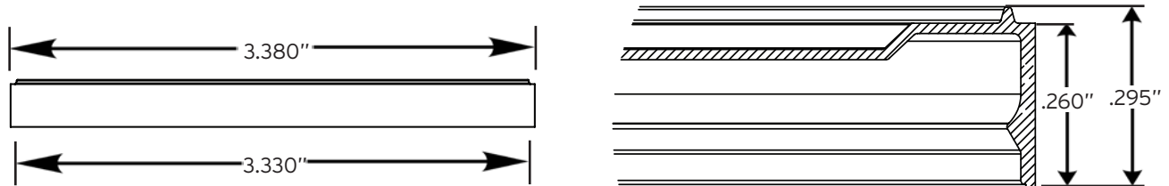
Side View
